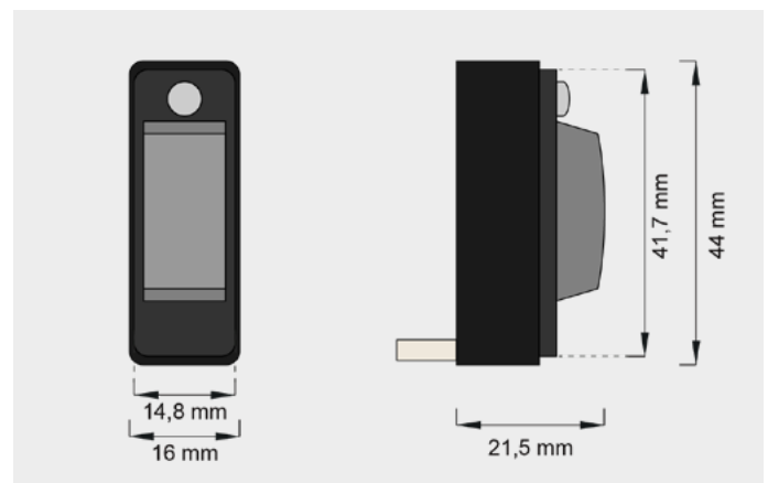
Dimensions of sensor
